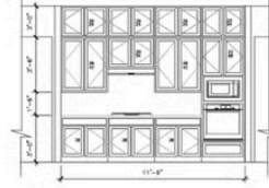
J KITCHEN UPPER CABS (OPT.)
