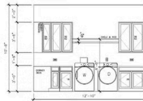
D LAUNDRY (OPT.)
