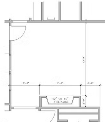
C LIVING ROOM FIREPLACE (OPTION) FIRE PLACE OPTION
