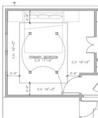
A PRIMARY BEDROOM LIGHT & TRAY CEILING OPTION
