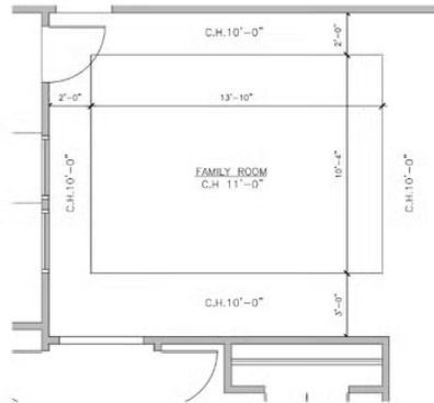
B FAMILY ROOM (OPTION) TRAY CEILING OPTION
