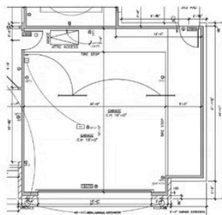
F 5' GARAGE EXTENSION (OPTION)
