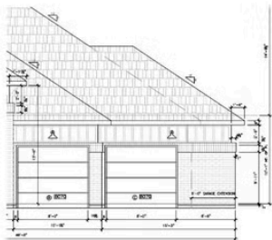
D 5' GARAGE EXTENSION (OPT.)
