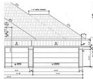
E 3 CAR GARAGE (OPT.)
