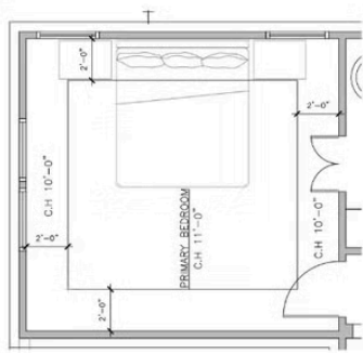
A PRIMARY BED CEILING (OPT.)
