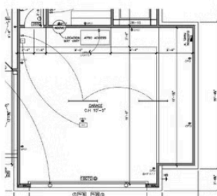
H 5' GARAGE EXTENSION (OPTION)
