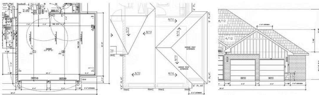
A 5' GARAGE EXTENSION (OPTION)
