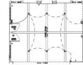
J LIVING ROOM BEAMS (OPTION)
