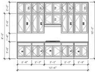
A KITCHEN (OPTION)
