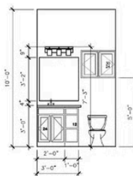
C BATH #2 (OPTION)
