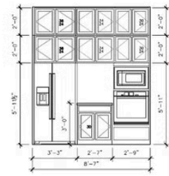
B KITCHEN (OPTION)
