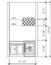
F BUILT-IN CABINET WINE BAR
