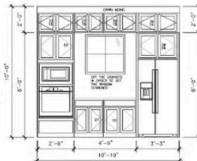
K KITCHEN (OPT.)
