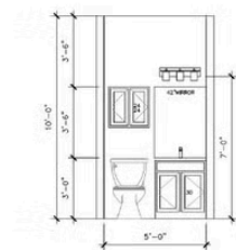
I POWDER BATH (OPT.)
